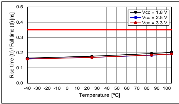
Rise Time
