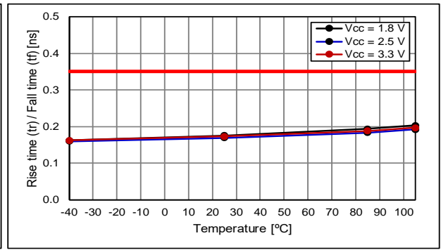
Fall Time
